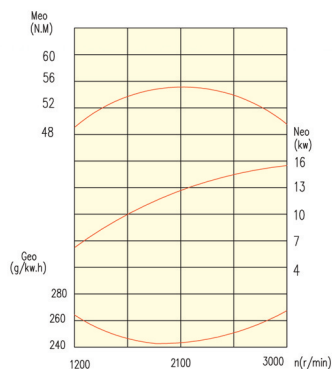
Full speed & full load characteristic curve Model 3M78 diesel engine
